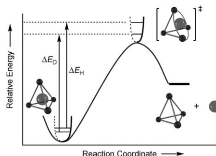
Figure 3. Proposed reaction coordinate diagram for the displacement of a guest from host 1 . An increase in guest C–H/D force constants when constricted at the sterically strained transition state drives the CH and CD ZPEs further apart relative to the ground state, thus resulting in a larger activation energy for the ejection of a protiated guest ( \Delta E_H > \Delta E_D ).
